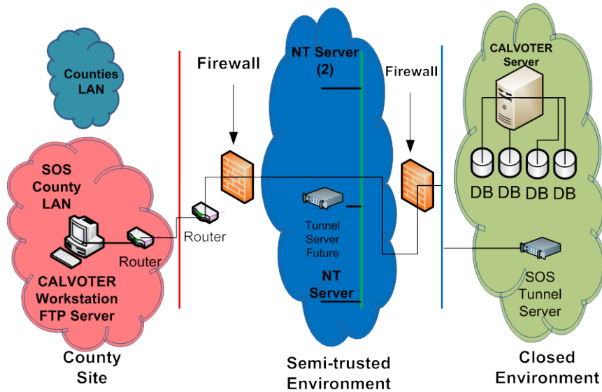
Figure III.9 – Calvoter Security Architecture
